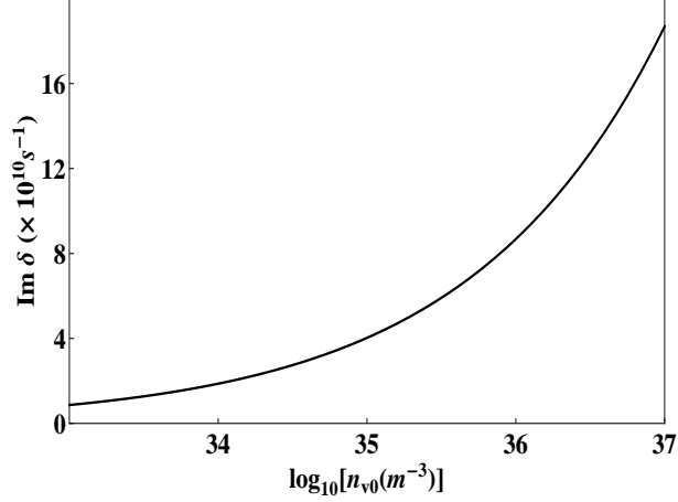
FIG. 2: Instability growth rate from Eq. (30) for \mathcal{E}_{\nu 0} = 10 \text{ MeV} , v_T/c = 1/10 , n_0 = 10^{34} \text{ m}^{-3} , B_0 = 5 \times 10^7 \text{ T} , as a function of neutrino beam number density n_{\nu 0} , for \mathbf{k} \perp \boldsymbol{\omega}_c .
