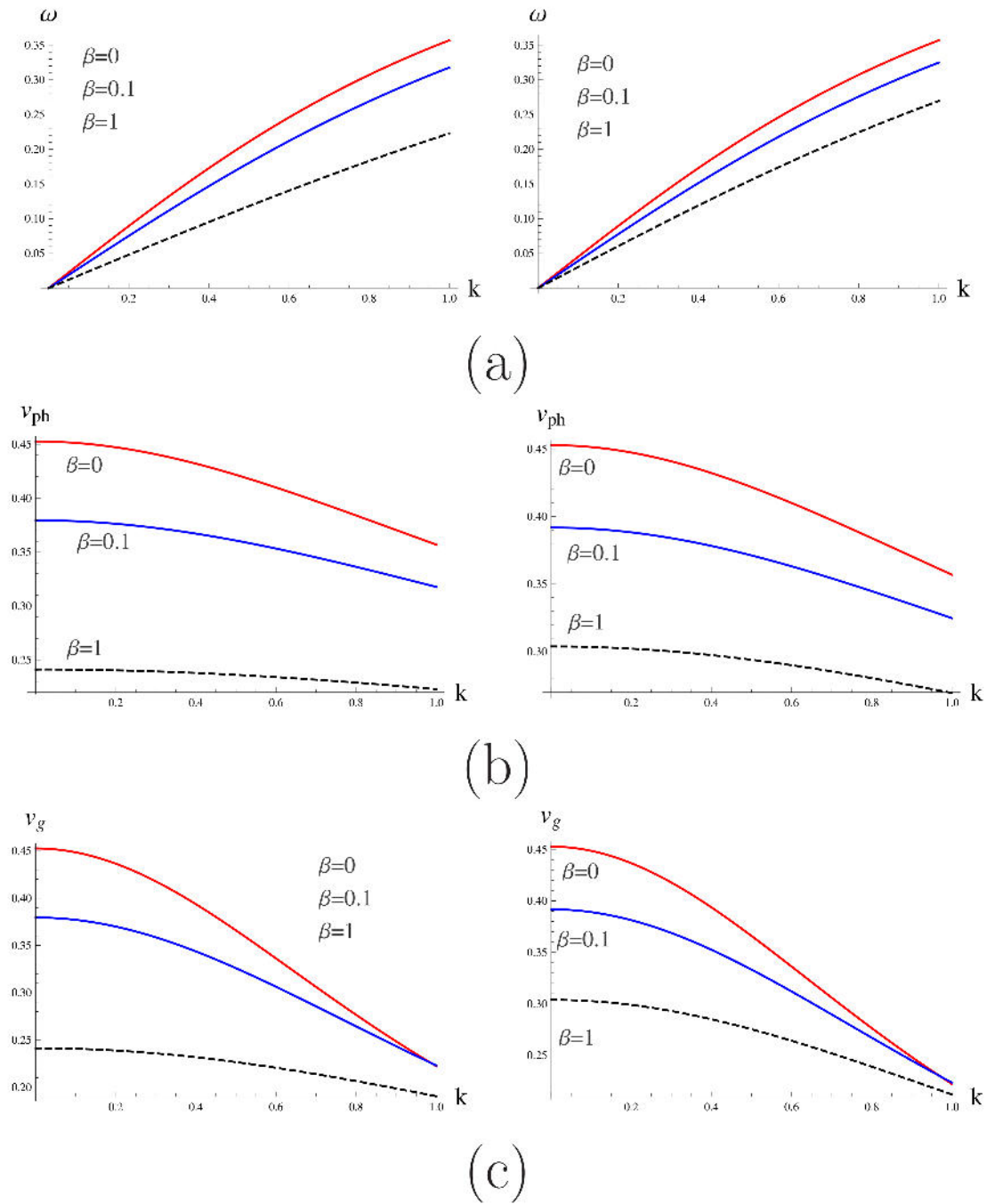
Figure 1. Illustrative plots of the frequency, the phase speed, v_{ph} = \omega/k , and the group velocity, v_g = d\omega/dk , versus the wavenumber k , for different values of the positron-ion charge density ratio, \beta . The parameter values in this plot have been arbitrarily chosen so that ab = 1/3 , n_{i0} = 10^{33} and T_e = T_p = 10^7 K . The plots to the right are made with fixed scales (corresponding to a reference density n_c = 10^{33} m^{-3} , cf. discussion in Sec. 7).
