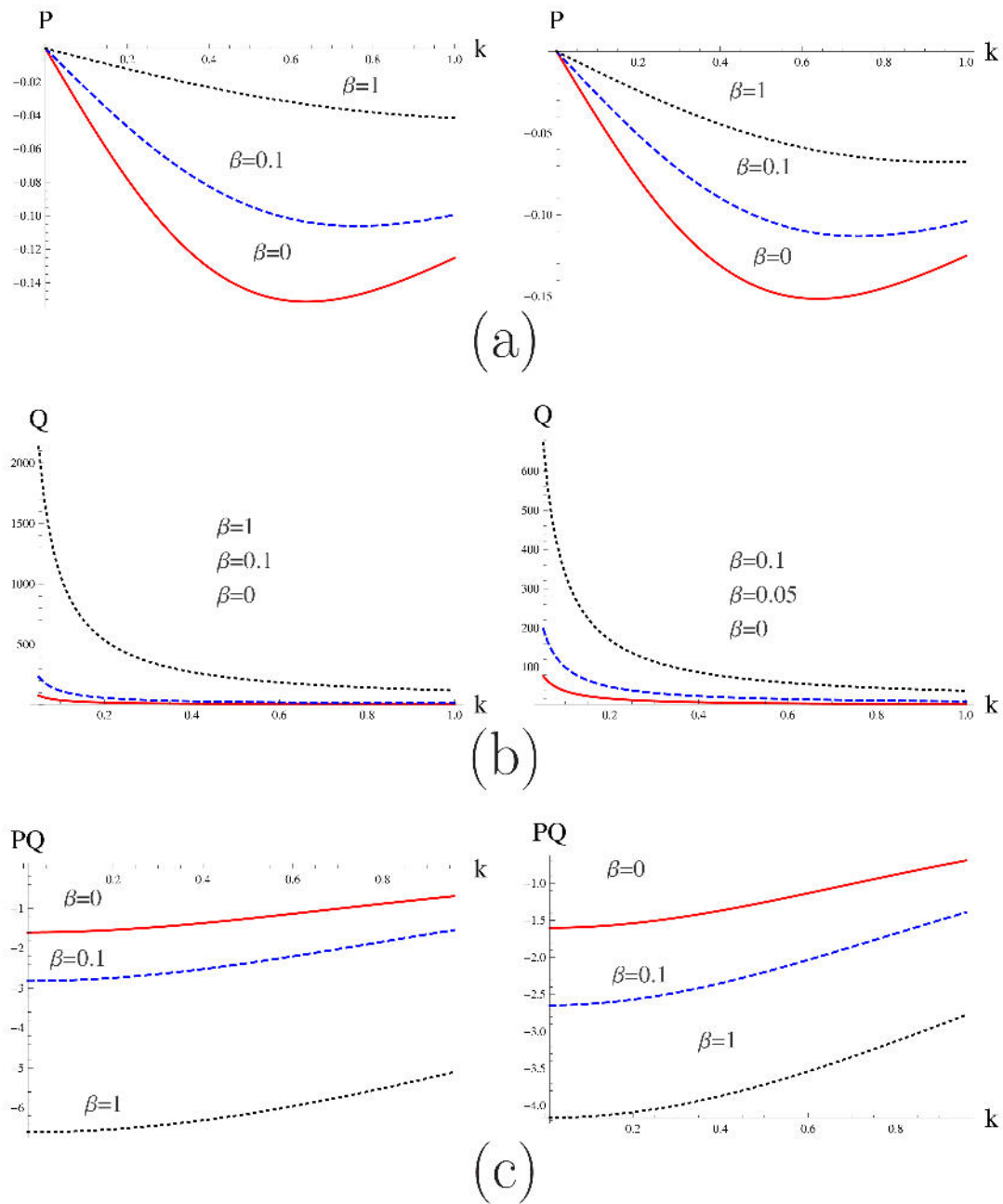
Figure 3. The effect of positron population ( \beta = \frac{n_{p0}}{n_{i0}Z_i} ) on P , Q and on their product PQ is shown above (with T_e = T_p ), in panels (a), (b) and (c), respectively. Recall that the region PQ > 0 admits unstable harmonic (and stable bright-type envelope soliton) solutions of the NLSF. The plots to the right were made with a fixed scale (cf. discussion in Sec. 7).
