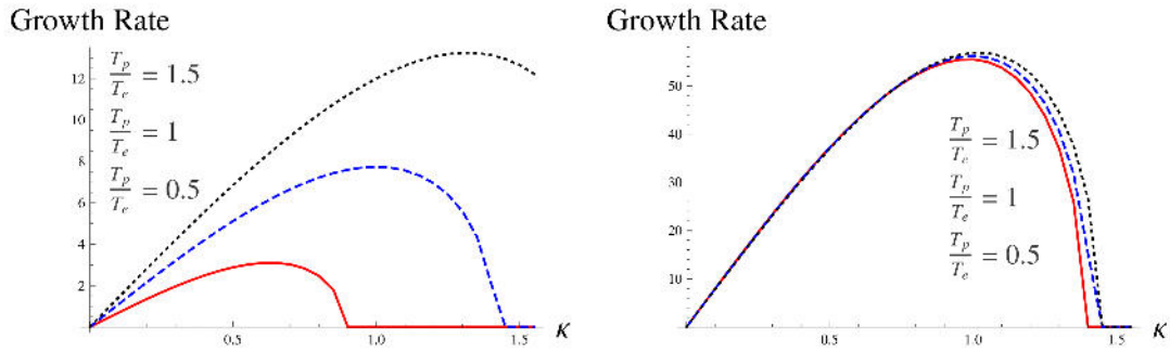
Figure 6. The modulational instability growth rate is depicted as a function of perturbation wavenumber, \kappa , for different positron temperatures. \kappa is in units of \kappa_{max} for T_p = T_e . k = 3.5 for all three curves. The plot to the right was made with a fixed scale (cf. discussion in Sec. 7).
