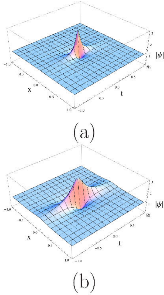
Figure 17. Peregrine's solution is depicted for two values of \beta . The first figure has k = 2.5 , T_p/T_e = 1 and \beta = 0 , whereas \beta = 0.1 in the second, which is of greater duration and spatial extension (i.e. less localized).
