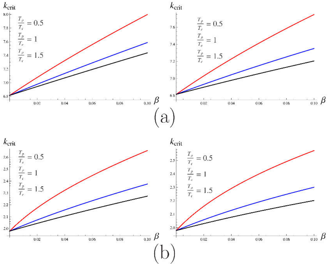
Figure 8. For large k ( k = 2.3 in this plot), solutions are unstable for small \beta .
