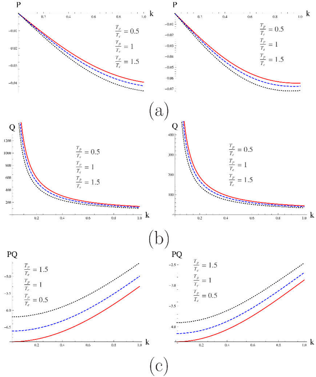
Figure 4. The effect of electron-positron temperature ratio on P , Q , PQ is shown above for \beta = 1 . The curve in red shows Q with T_p/T_e = 0.5 ; the blue, dashed curve is for T_p/T_e = 1 ; and the black, dotted curve is for T_p/T_e = 1.5 . The plots to the right were made with a fixed scale (cf. discussion in Sec. 7).
