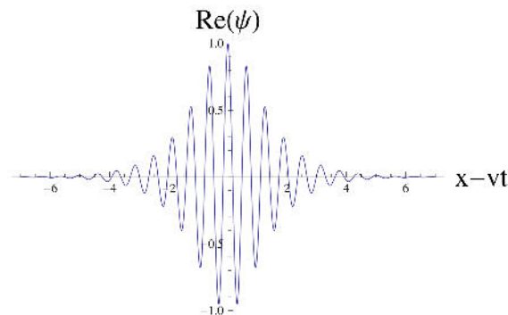
Figure 11. The bright envelope soliton amplitude varies roughly as \text{sech}(x - vt) .
