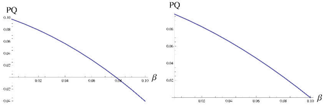
Figure 8. For large k ( k = 2.3 in this plot), solutions are unstable for small \beta .
