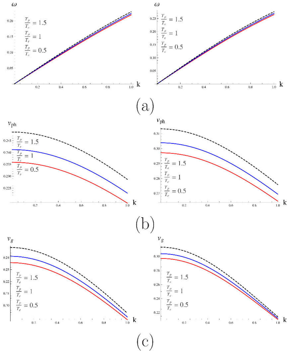
Figure 2. Illustrative plots of the frequency, the phase speed and the group velocity, versus the wavenumber for different positron temperatures with fixed electron temperature. The parameter values in this plot have been arbitrarily chosen so that ab = 1/3 , n_{i0} = 10^{33} , T_e = 10^7 K and \beta = 1 . The plots to the right are made with fixed scales (corresponding to a reference density n_e = 10^{33} m^{-3} ; cf. discussion in Sec. 7).
