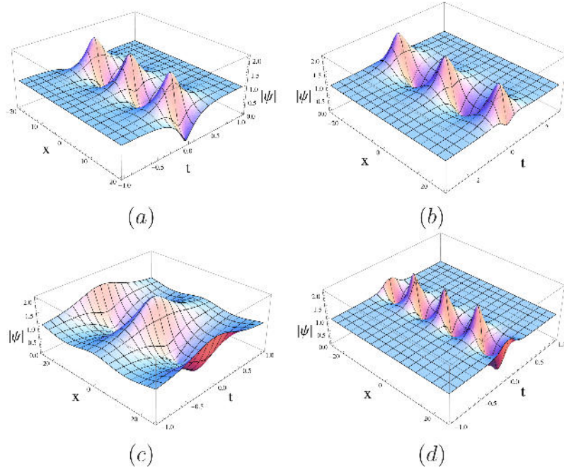
Figure 19. Plots of Akhmediev's breather for different values of \beta and T_c/T_p : (a), (b) k = 2.5 , T_p/T_c = 1 , \beta = 0, 0.1 ; (c), (d) k = 3.5 , \beta = 1 , T_p/T_c = 0.5, 1.5 .
