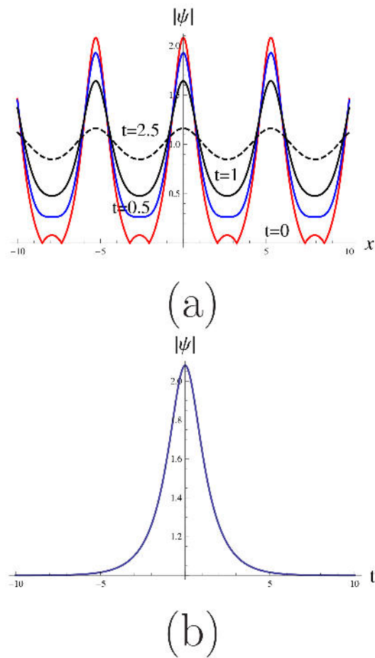
Figure 14. As suggested by (42), the Akhmediev breather is periodic in space, but not in time.
