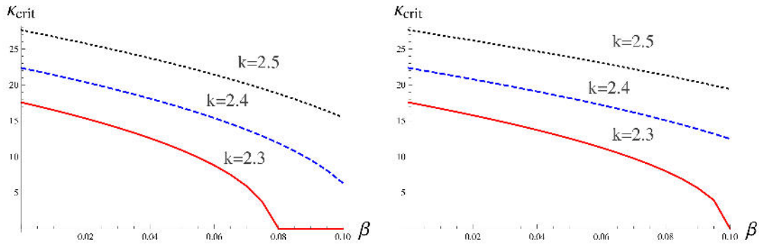
Figure 7. An increase in positron population affects the stability threshold (40) as shown above. The plot to the right was made with a fixed scale (cf. discussion in Sec. 7).
