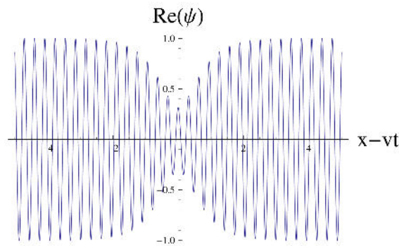
Figure 12. Heuristic plot of the grey-type envelope soliton, whose amplitude varies roughly as [1 - d^2 \text{sech}^2(x - vt)]^{1/2} . Setting d = 1 results in a dark-type envelope soliton.
