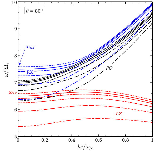
FIG. 8. Same as Figs. 6 and 7, but with propagation angle \theta = 80^\circ .
