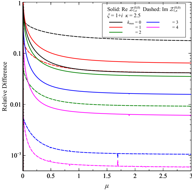
FIG. 4. Same as Fig. 3, but for n = 1 .
