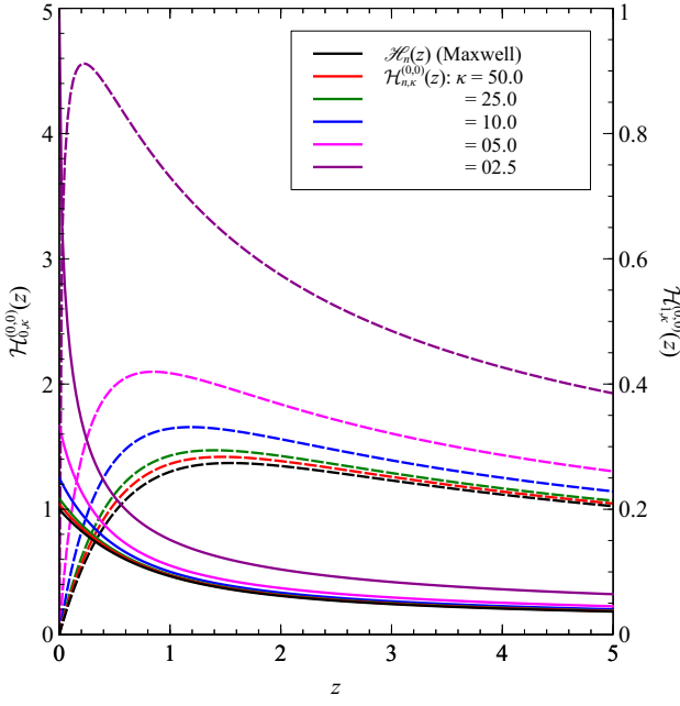
FIG. 1. Plots of function \mathcal{H}_{n,\kappa}^{(0,0)}(z) for n = 0 (full lines) and n = 1 (dashed lines) and several values of the \kappa parameter. The limiting form \mathcal{H}_n(z) for \kappa \rightarrow \infty is also included.
