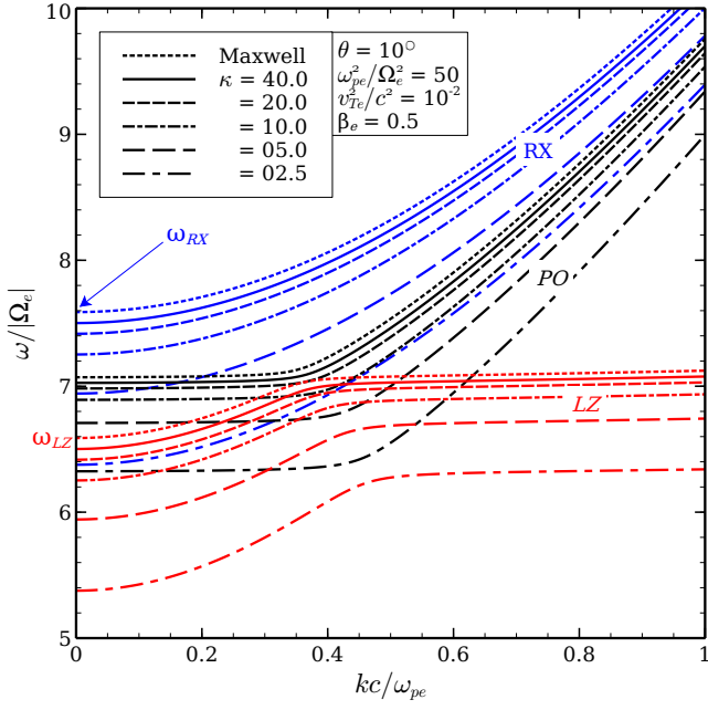
FIG. 6. Plots of high-frequency dispersion relations in a high-beta, kappa plasma, as the numerical solutions of the dispersion equation (9), for propagation angle \theta = 10^\circ . The dispersion equation is solved for several values of the \kappa parameter, including the limit \kappa \rightarrow \infty (Maxwell). The modes with elliptic polarization are named: RX (right-fast extraordinary), PO (plasma-ordinary) and LZ (left-slow extraordinary).
