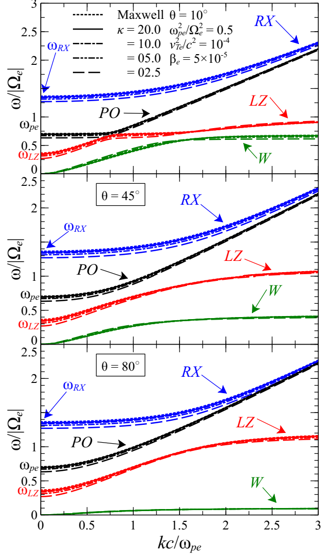
FIG. 5. Plots of high-frequency dispersion relations in a low-beta, kappa plasma, as the numerical solutions of the dispersion equation (9), for propagation angles \theta = 10^\circ , 45^\circ and 80^\circ . For each angle, the dispersion equation is solved for several values of the \kappa parameter, including the limit \kappa \rightarrow \infty (Maxwell). The modes with elliptic polarization are named: RX (right-fast extraordinary), PO (plasma-ordinary), LZ (left-slow extraordinary) and W (whistler).
