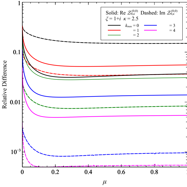
FIG. 3. Plots of the real (solid lines) and imaginary (dashed) parts of the relative difference \Delta between functions \mathcal{Z}_{\text{sum}} and \mathcal{Z}_{\text{int}} for n = 0 , \alpha = \beta = 0 , \kappa = 2.5 , \xi = 1 + i and different values of k_{\text{max}} .
